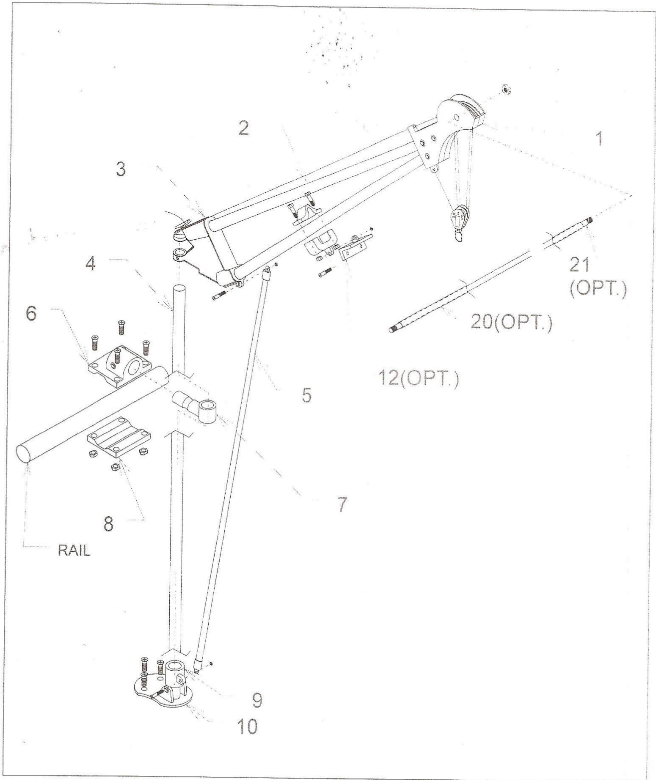
ASSEMBLY DRAWING- MODEL 1200- SYSTEM A1
